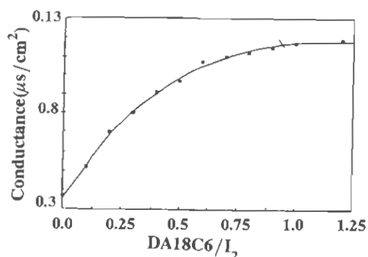
Fig. 3: Plot of conductance vs. DA18C6/I 2 mole ratio in acetonitrile for a 1.77 \times 10^{-1} mM iodine obtained at 25°C
