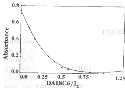
Fig. 2: Plot of absorbance vs. DA18C6/ \text{I}_2 mole ratio in acetonitrile for a 2.91 \times 10^{-2} mM iodine obtained at 364 nm and 25^\circ\text{C} .
