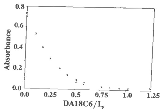
Fig. 4: Computer fit of the plot of absorbance vs. DA18C6/I 2 mole ratio obtained at 364 nm and 25°C: (x) experimental points; (o) calculated points; (=) experimental and calculated points are the same within the resolution of plot.
