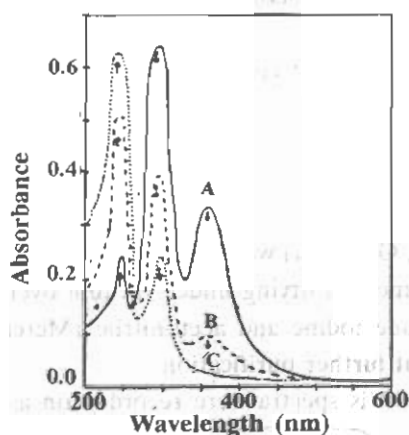
Fig. 1: Absorption spectra of a 1.33 \times 10^{-2} mM iodine in the presence of 0 (A), 0.25 \times 10^{-2} (B) and 0.88 \times 10^{-2} (C) mM DA18C6 in acetonitrile solution.
