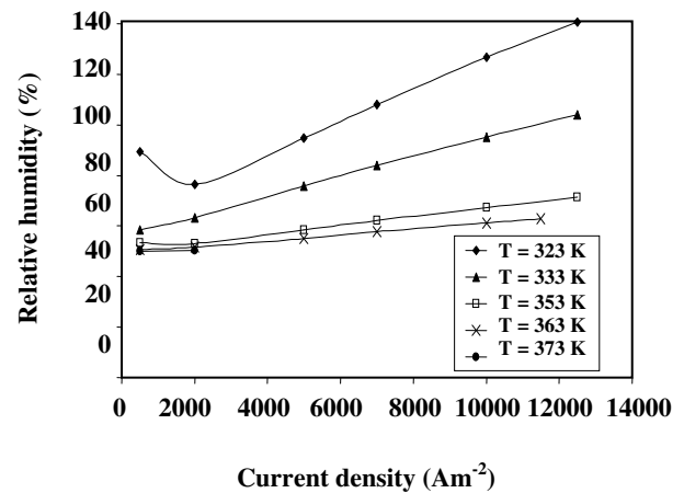
Fig. 12: Maximum relative humidity within cathode GDL versus current density for various temperatures of channels fluid.
