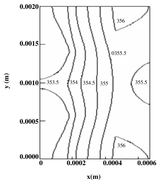
Fig. 5: Temperature (K) contours.
