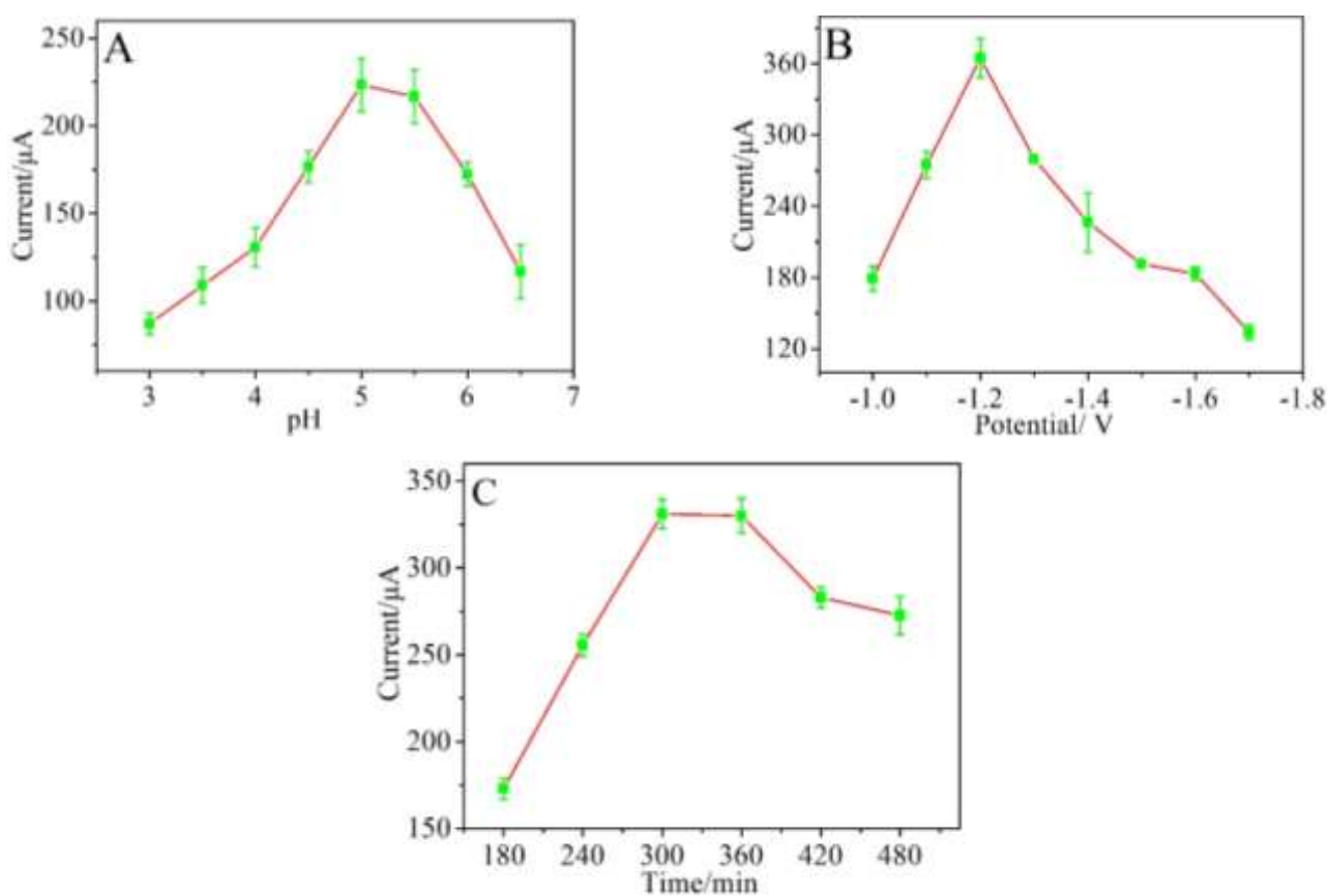
Fig. S2: Effect of pH value (A), deposition potential (B) and deposition time (C) on the anodic peak responses for 100 \mu\text{M} Pb(II) at the MWCNTs-TPI-2-Ph electrode.
