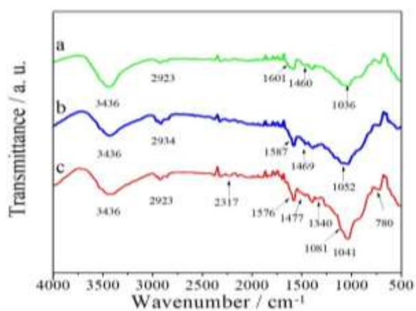
Fig. S1: FTIR spectra of MWCNTs-COOH (a), MWCNTs-OH (b), and MWCNTs-TPI-2-Ph (c).
