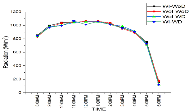
Fig. 7: Variation of solar intensity with local time for different combinations
