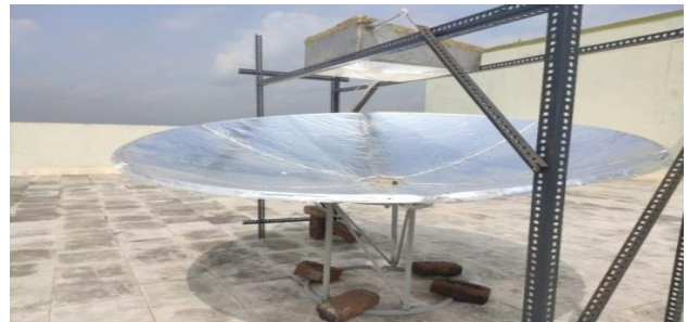
Fig. 4: Solar still without insulation and with dish (WoI-WD)
