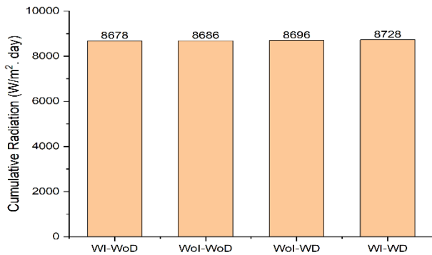
Fig. 8: Cumulative daily solar intensity for different combinations
