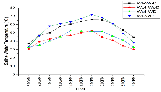
Fig. 9: Variation of saline water temperature with time
