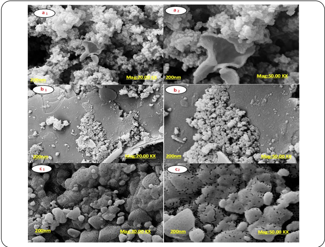
Fig. 3: SEM spectra of a) MNPs, b) MNPsH3 and c) DS loaded MNPsH3.
