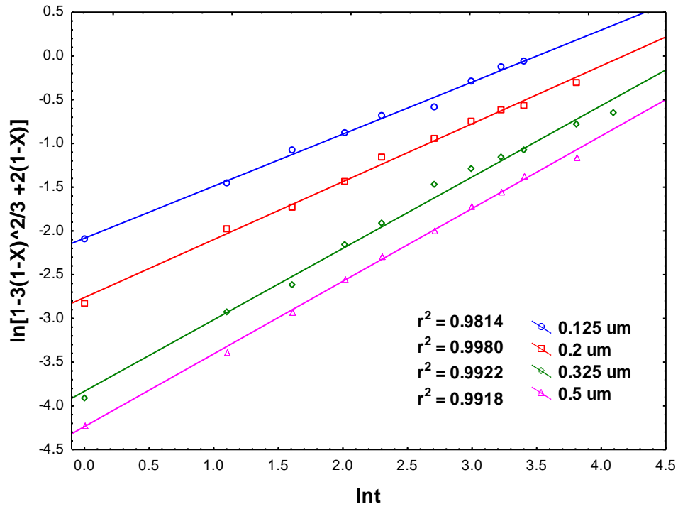
Fig. 14: Variation of \ln[1 - 3(1-X)^{2/3} + 2(1-X)] against Int for different particle sizes
