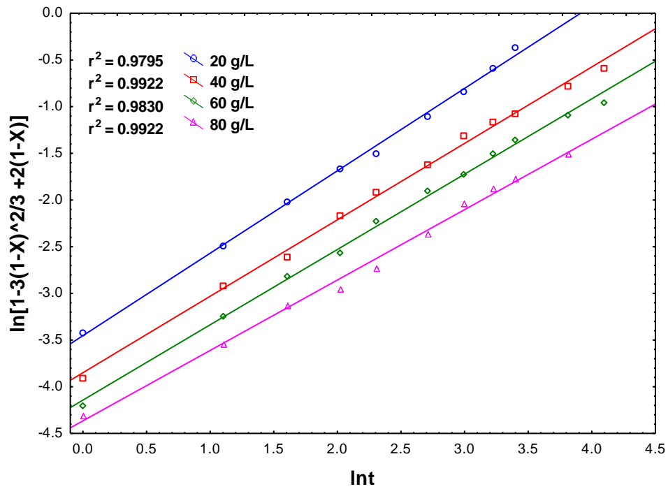
Fig. 15: Variation of \ln[1 - 3(1-X)^{2/3} + 2(1-X)] against Int for different solid-liquid ratios
