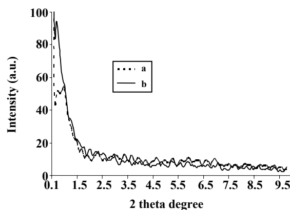
Fig. 3: Low-angle XRD pattern of synthesized (a) and calcined \text{TiO}_2 (b).
