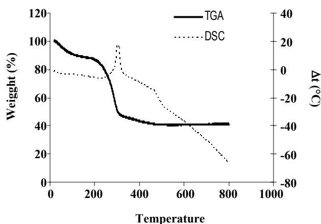
Fig. 5: TG-DSC curves for the TiO 2 before calcinations.
