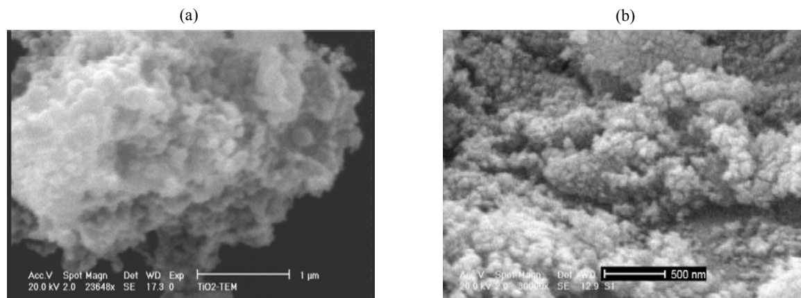
Fig. 4: SEM images of synthesized TiO 2 after calcination at scale 1 μm (a) and 500 nm (b).
