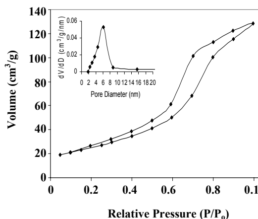
Fig. 6: N 2 -adsorption-desorption isotherms, and inset: BJH pore size distribution curve of prepared mesoporous TiO 2 .
