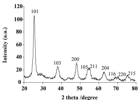
Fig. 2: Wide- angle XRD patterns of the calcined \text{TiO}_2 sample (with anatase lines shown for reference).
