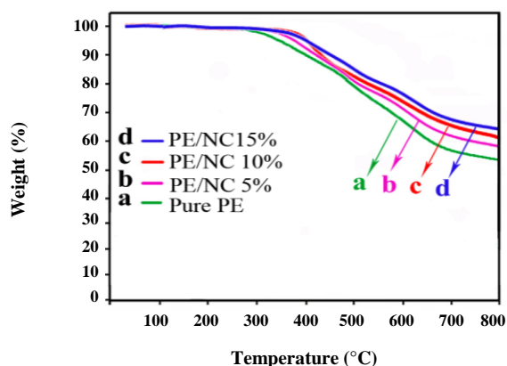
Fig. 3: TGA thermograms of pure PE (a) PE/SiO 2 NC 5%, (b) PE/SiO 2 NC 10%, (c) PE/SiO 2 NC 15%, (d).
