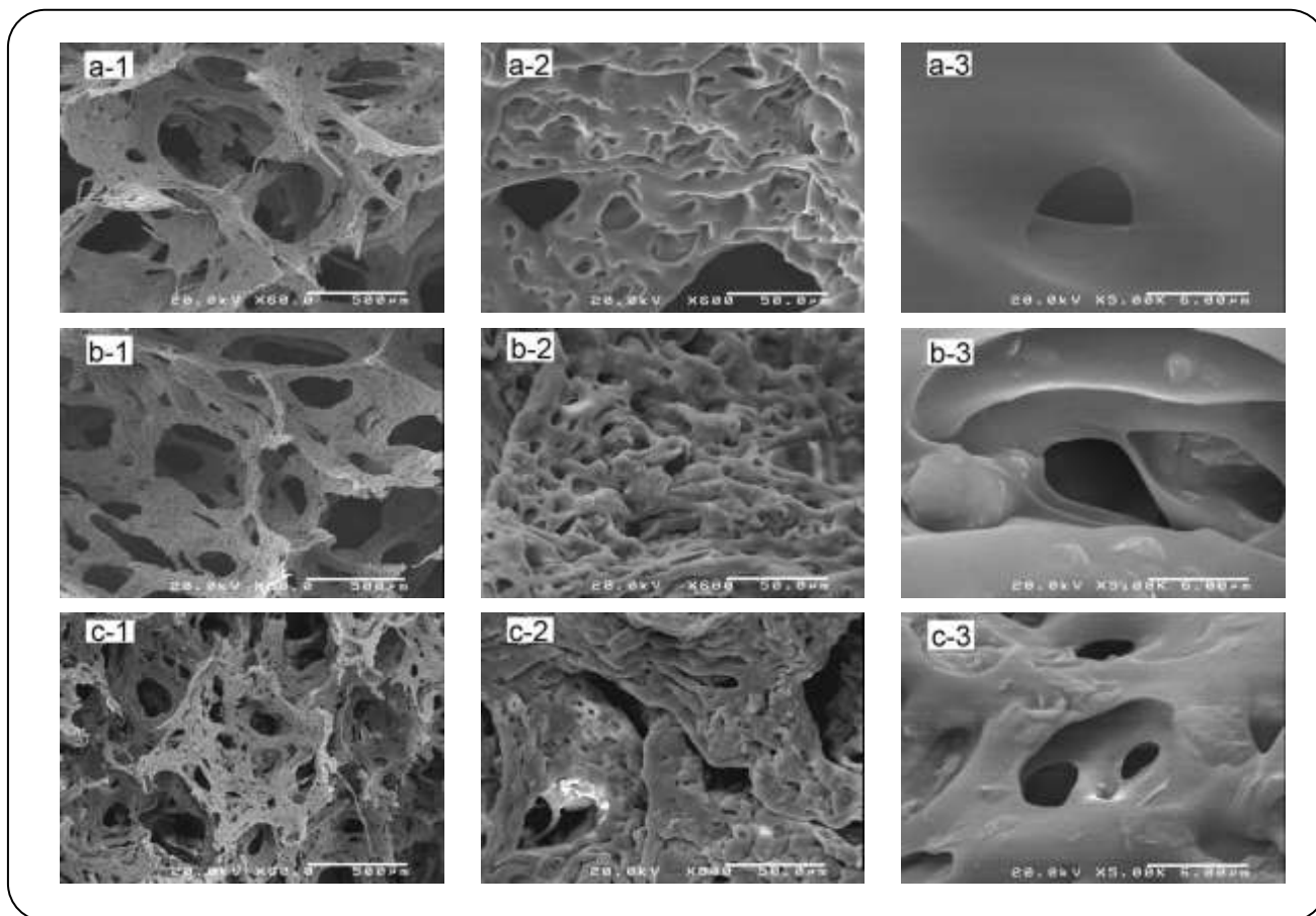
Fig. 5: FESEM images of (a-1 to a-3) PVA, (b-1 to b-3) PVA/Cl and (c-1 to c-3) PVA/ N1 foam samples with three different magnifications. Magnification factors are specified at the bottom of the images.
