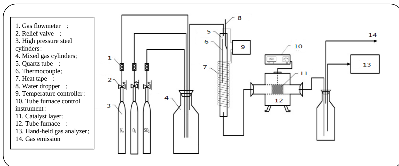
Figure.1 The testing device of modified pyrolysis tar performance
