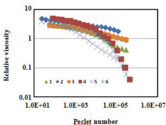
Fig. 6: Relative viscosity of emulsions containing of TG and WPI plotted as relative viscosity as function of pecelet number (Numbers refer to formulations in Table 1).
