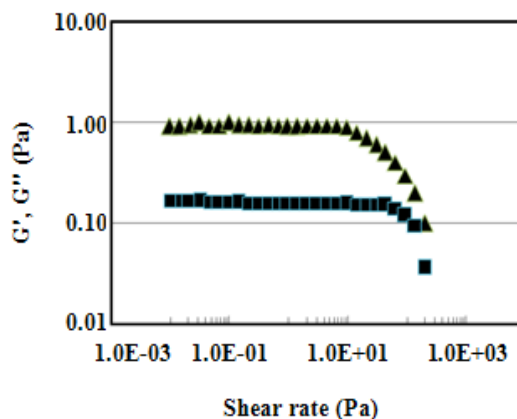
Fig. 10: Amplitude sweep test of 0.5% Gum, 4% WPI and 5% Oleic acid.
