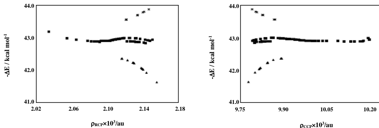
Fig. 4: The binding energies of the \text{Na}^+ -graphene and \text{Na}^+ -SWCNTF complexes versus \rho_{RCP} s at the central rings of the graphene sheet and SWCNTFs (a) and versus \rho_{CCP} s (b) for the first (■), second (▲), and third (×) brands.
