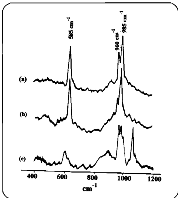
Fig.2: Raman spectra of three glass-ceramic samples prepared by the sol-gel method in the wavenumber shift range 400-1200 \text{cm}^{-1} .
