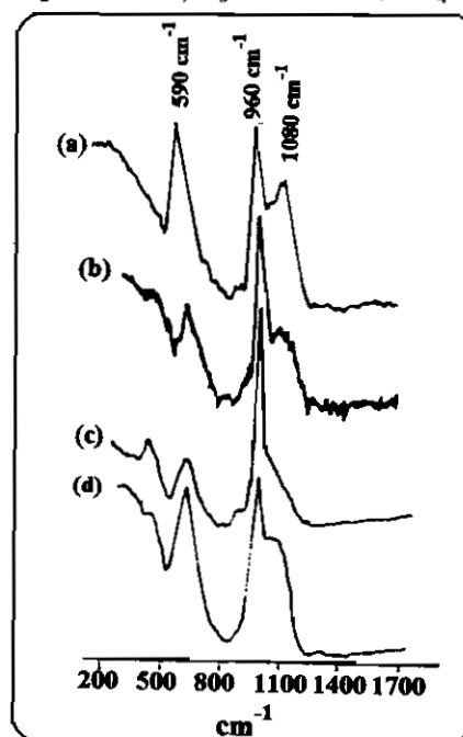
Fig.1: Raman spectra of four glass-ceramic samples prepared by the heat treatment method in the wavenumber shift range 200-1700 cm -1 .
