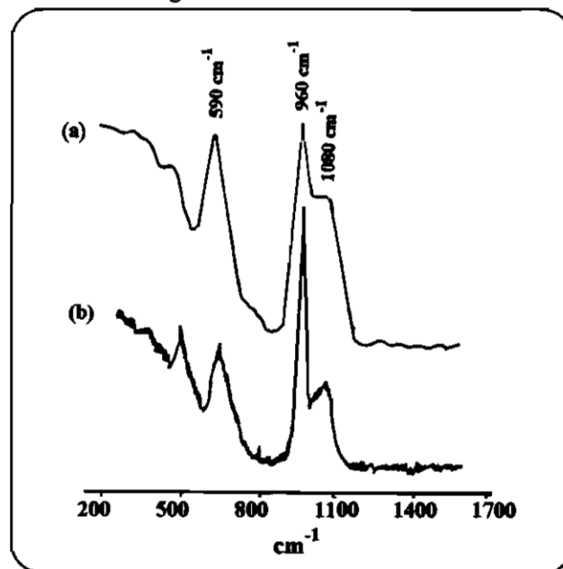
Fig.3: Raman spectra of a sample of glass-ceramic prepared by the heat treatment method before (a) and after (b) immersion in SBF solution in the wavenumber shift range 200-1700 \text{cm}^{-1} .
