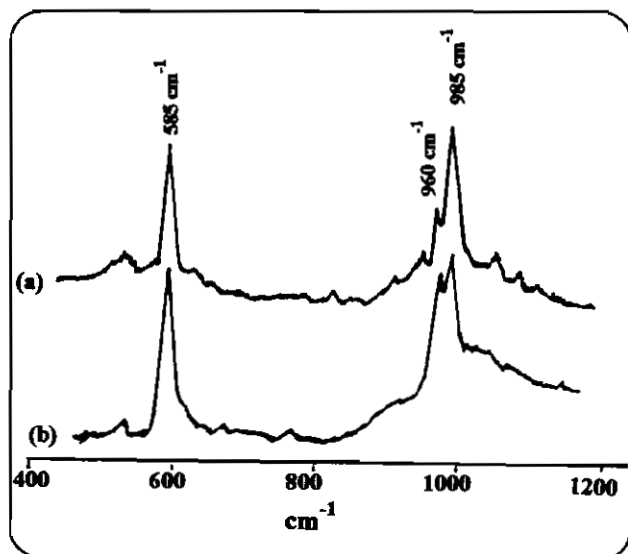
Fig.4: Raman spectra of a sample of glass-ceramic prepared by the sol-gel method before (a) and after (b) immersion in SBF solution in the wavenumber shift range 400-1200 \text{cm}^{-1} .
