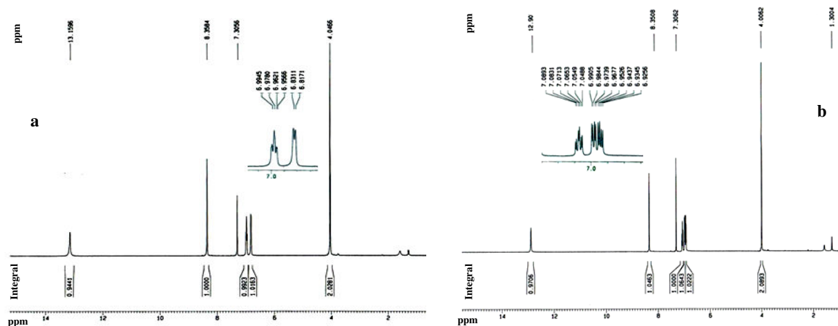
Fig. 2: 1 H NMR spectra (CDCl 3 , 500 MHz) of 3b (a) and 3c (b) compounds.
