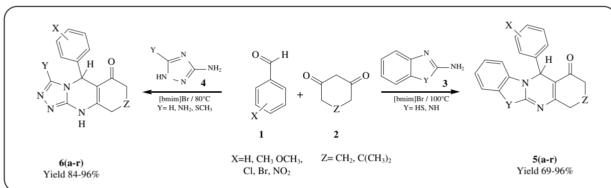
Scheme 2: Synthesis of tetrahydrobenzimidazo[2,1- b ]quinazolin-1(2 H )-ones (5 a-r ) and tetrahydro-1,2,4-triazolo[5,1- b ]quinazolin-8(4 H )-ones (6 a-r )
