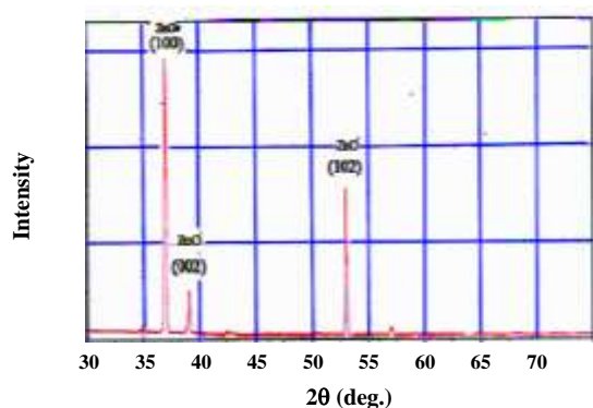
Fig. 5: X-ray diffraction pattern of ZnO NPs in NaOH(0.1M). \lambda=532\text{nm} .
