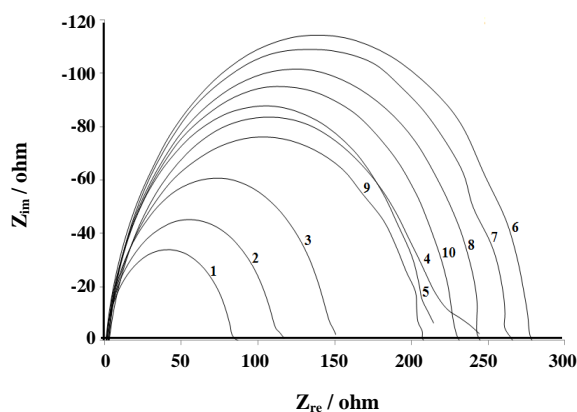
Fig. 4: The effect of immersion time on mild steel in 1 M HCl in the presence of 2 \times 10^{-4} M inhibitor: (1) 30 min, (2) 1h, (3) 4 h, (4) 8 h, (5) 12 h, (6) 16 h, (7) 20 h, (8) 24 h, (9) 26 h and (10) 30 h.
