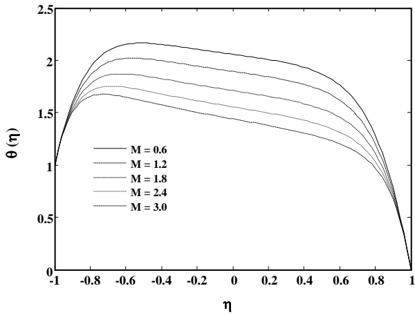
Fig. 12: Variation of temperature for R = 5, \alpha = 1, C_1 = 1.4, C_2 = 0.7, C_3 = 1, Ec = 1.6, \epsilon = 1, Nr = 0.2, Pr = 1.7 and various M .
