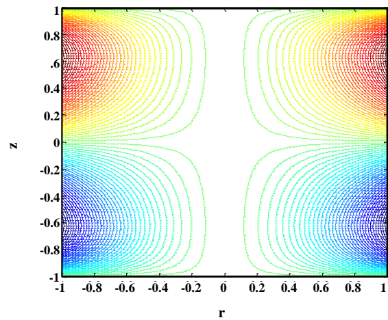
Fig. 1: a) Physical Configuration of the problem. b) Streamlines for the flow for M=1, \alpha=1, C_1=1, C_2=0.2, C_3=0.3, Ec=1, \epsilon=1, Nr=1, Pr=1 .
