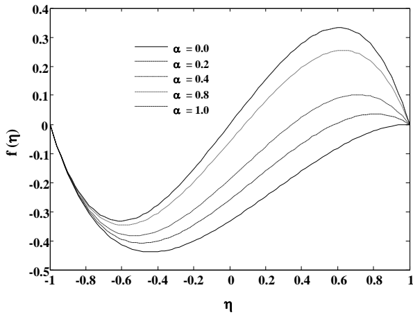
Fig. 18: Variation of axial velocity for R = 4, Ec = 1.6, C_1 = 1.4, C_2 = 0.7, C_3 = 1, Pr = 1.7, M = 0.5, \epsilon = 1, Nr = 0.3 and various \alpha .
