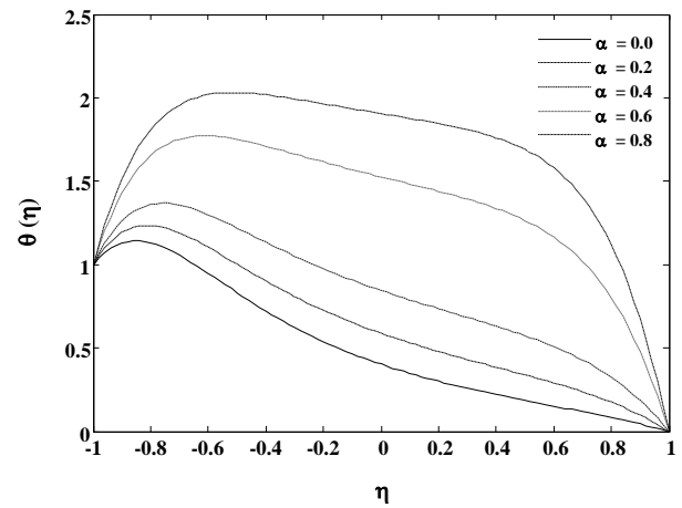
Fig. 21: Variation of temperature for R = 4, Ec = 1.6, C_1 = 1.4, C_2 = 0.7, C_3 = 1, Pr = 1.7, M = 0.5, \epsilon = 1, Nr = 0.3 and various \alpha .
