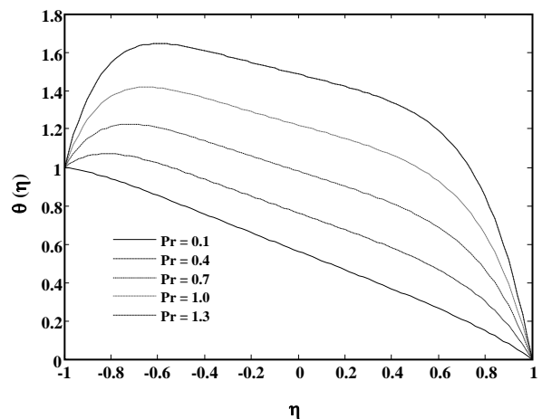
Fig. 17: Variation of temperature for R = 5, \alpha = 1, C_1 = 1.4, C_2 = 0.7, C_3 = 1, Ec = 0, M = 0.5, \epsilon = 1, Nr = 0.2 and various Pr .
