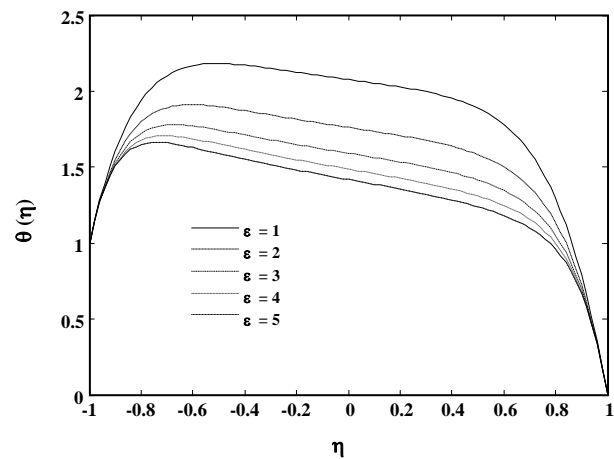
Fig. 16: Variation of temperature for R = 5, \alpha = 1, C_1 = 1.4, C_2 = 0.7, C_3 = 1, Ec = 1.6, M = 1.5, Nr = 0.2, Pr = 1.7 and various \epsilon .
