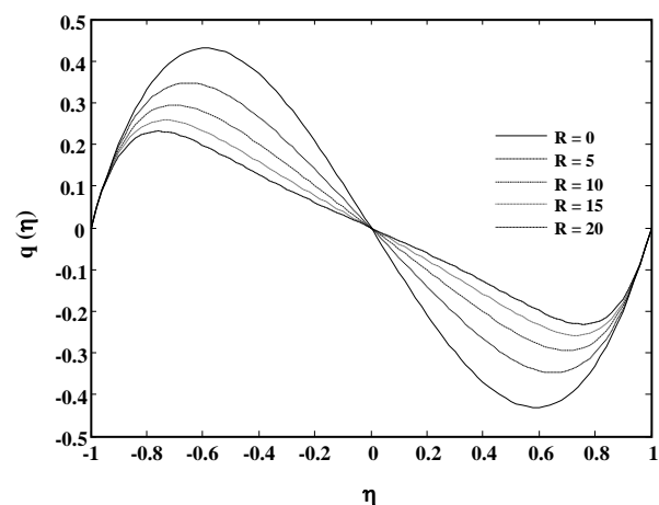
Fig. 5: Variation of microrotation for M = 0.5 , \alpha = 1 , C_1 = 1.4 , C_2 = 0.7 , C_3 = 1 , Ec = 1.6 , \varepsilon = 1 , Nr = 0.3 , Pr = 1.7 and various R .
