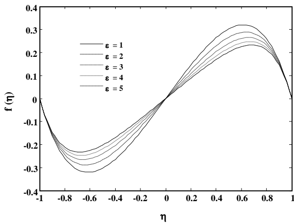
Fig. 13: Variation of temperature for R = 5, \alpha = 1, C_1 = 1.4, C_2 = 0.7, C_3 = 1, Ec = 1.6, M = 1.5, Nr = 0.2, Pr = 1.7 and various \epsilon .
