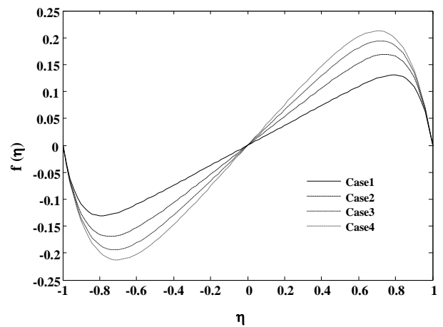
Fig. 22: Variation of axial velocity for R = 5, M = 5, \alpha = 1, Ec = 1.6, \epsilon = 1, Nr = 0.3, Pr = 1.7 and four cases of micropolar parameters.
