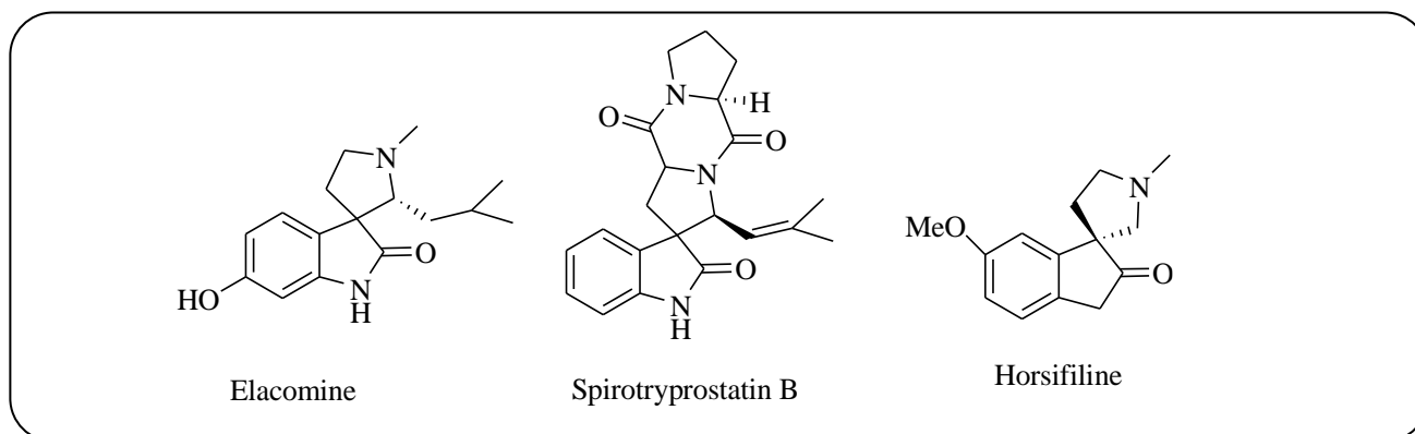
Fig. 1: Some alkaloids containing heterocyclic spirooxindole unit.
