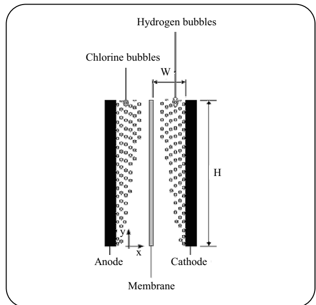
Fig. 1: Schematic sketch of the system considered.
