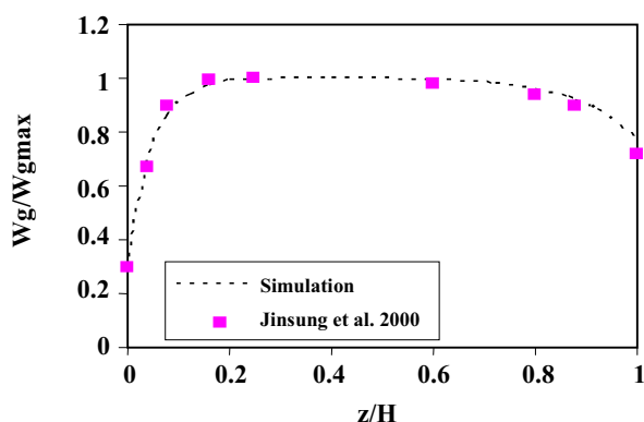
Fig. 3: Gas phase axial velocity along the centerline of vessel.
