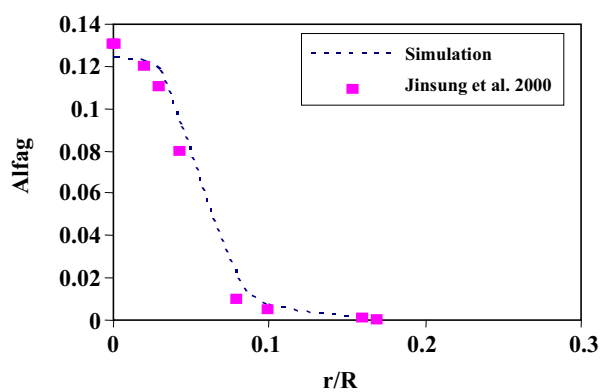
Fig. 6: Predicted gas void fraction distribution at the vertical section of z/H=0.36 .
