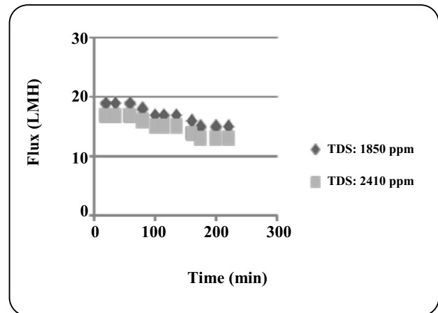
Fig. 9: Effect of feed concentration on fouling rate.
