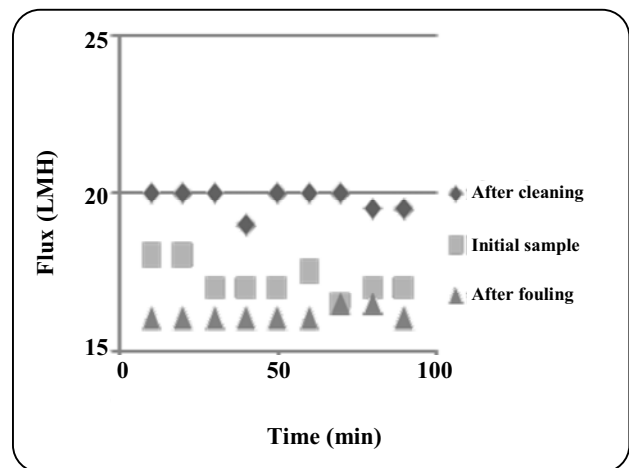
Fig. 10: Effect of cleaning on fouling rate.
