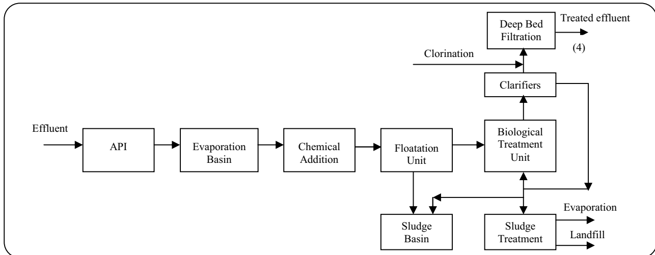
Fig. 1: Diagram of Tehran refinery wastewater treatment plant.
