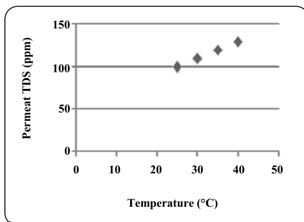
Fig. 6: Effect of temperature on permeate salinity (sample 1).
