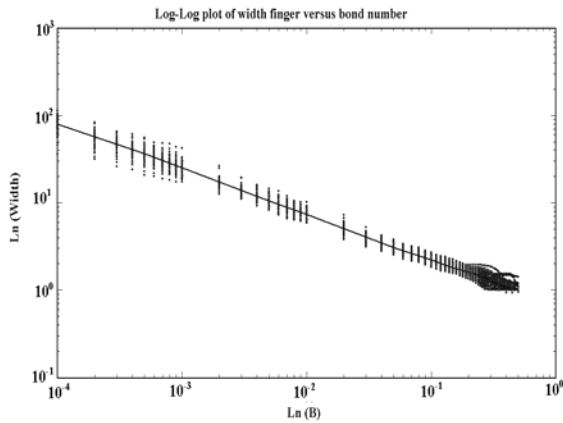
Fig. 9: Width of finger against bond number on log-log scale for 50 samples when oil injected from left edge. This shows that the slope is equal to -0.51.
