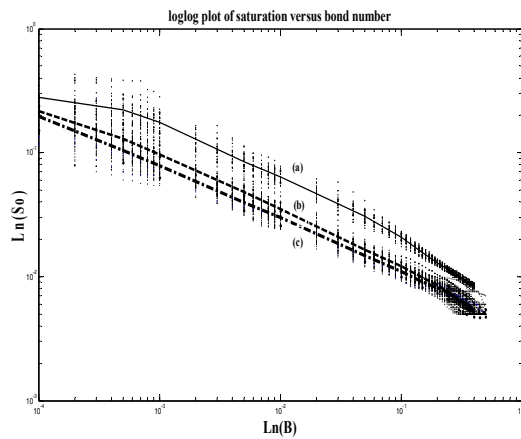
Fig. 12: Comparison of saturation slop respect to bond number on a log-log scale for uniform (solid line (a)), normal (dashed line (b)) and lognormal (dashed dot line(c)) distributions.
