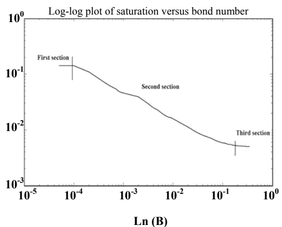
Fig. 7: Three zones for the saturation-bond number variations on a log-log scale.
