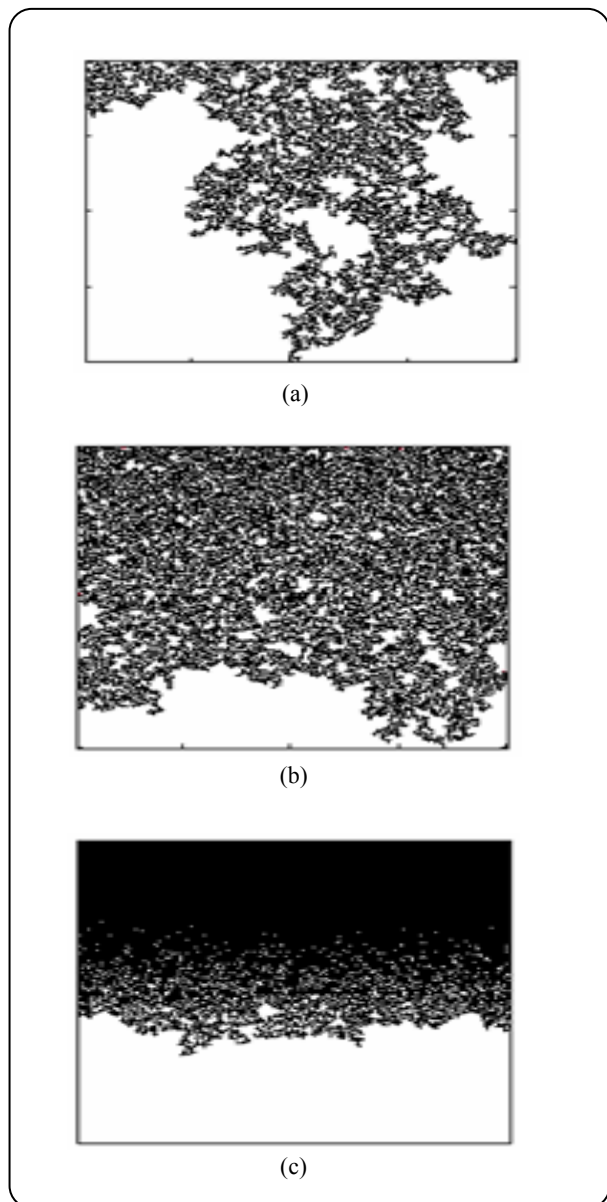
Fig. 3: Three realizations generated by the slow gravity stabilized displacement of a wetting fluid by a non wetting fluid in a quasi-two-dimensional porous medium in a lattice of size 200 \times 200 where (a) B=0 , (b) B=0.0001 , (c) B=0.001 .
