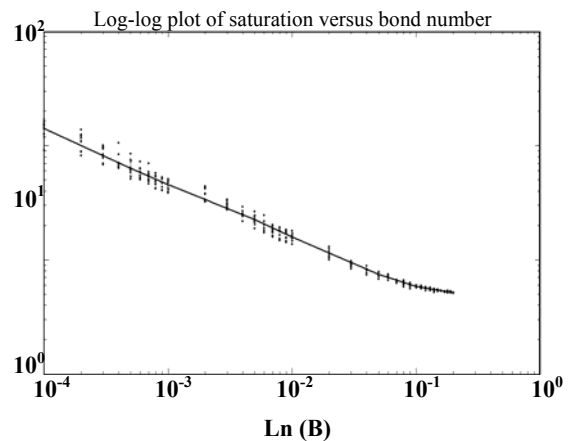
Fig. 6: Variation of saturation versus bond number on a log-log scale for 10 samples which shows a slope of -0.44.
