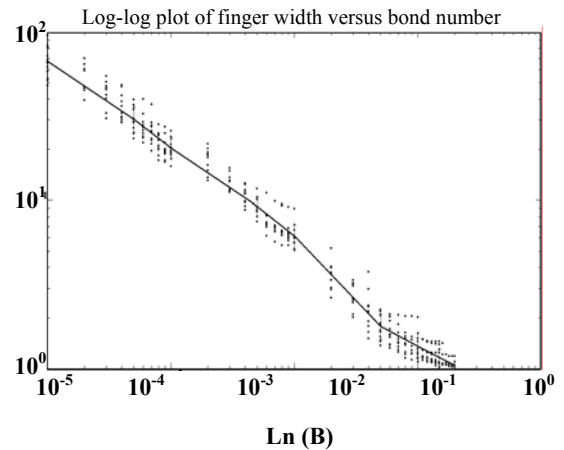
Fig. 5: Variation of width of finger versus bond number on a log-log scale for 10 samples which shows a slope of -0.58.
