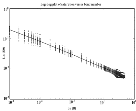
Fig. 10: Saturation against bond number on log-log scale for 50 samples when oil injected from left edge. This shows that the slope is equal to -0.44.
