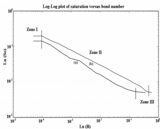
Fig. 11: Comparison of range of bond number in the case of injection of invader fluid from bottom of lattice (a) and in the case of injection of invader fluid from left side of lattice (b).
