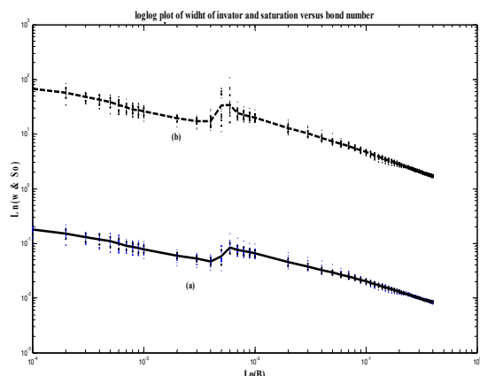
Fig. 15: Saturation (solid line (a)) and finger width (dashed line (b)) respect to bond number on a log-log scale for the composite lattice.
