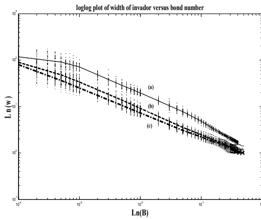
Fig. 13: Comparison of finger width slop respect to bond number on a log-log scale for uniform (solid line(a)), normal (dashed line (b)) and lognormal (dashed dot line(c)) distributions.
